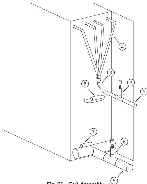
Fig. 01 - Coil Assembly
